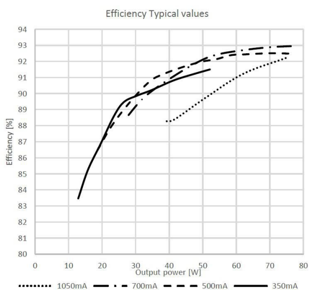
OT DX 75 G2 Typical Efficiency vs. Load (230 V 50 Hz)
