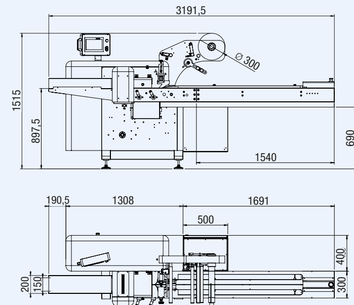
Layout SAROPACKER FlexFlow digit 400
