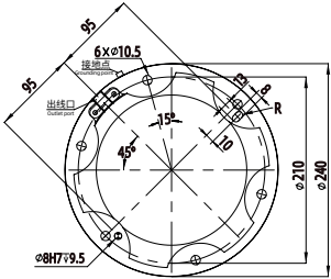
FR30 Pedestal diagram
