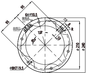
FR20 Pedestal diagram
