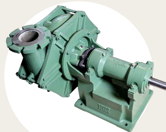
NPW 54 feed pump
