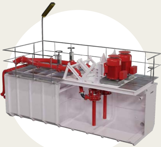
KBKM 150/400 dredger pump
