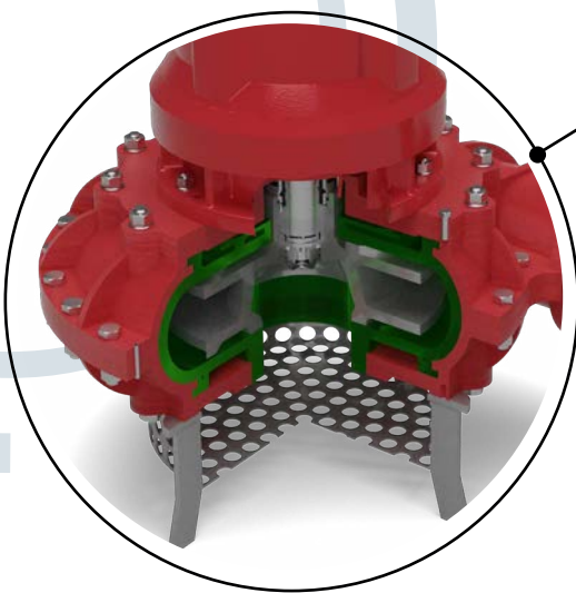
CRP PUMP WITH POLYURATHANE LINING
