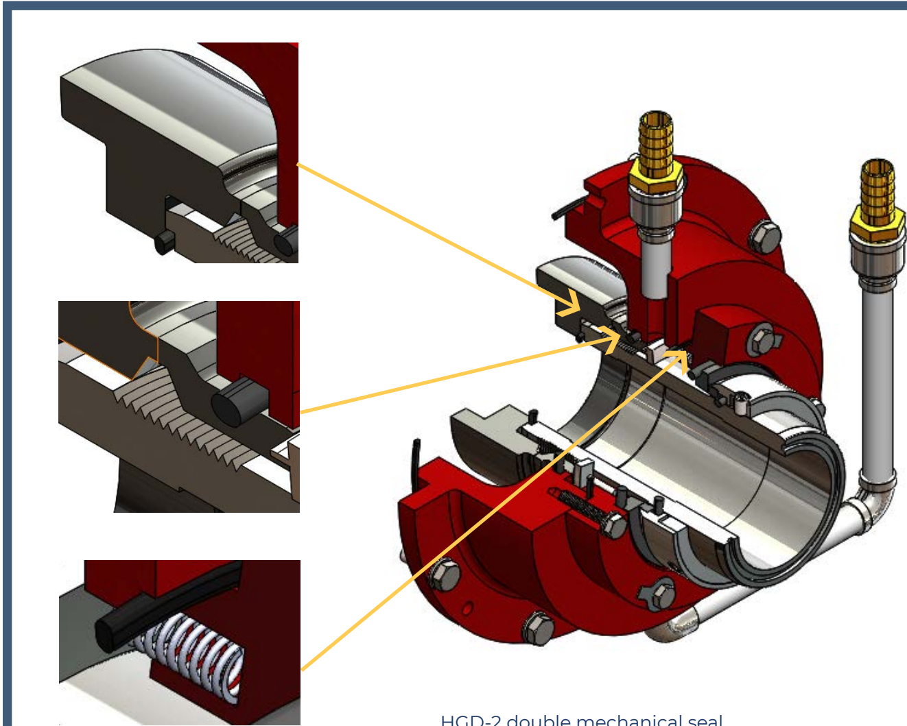
HGD-2 double mechanical seal with quench chamber
