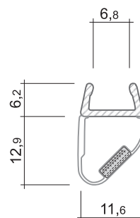
DD0116TR 2010 mm NS DD0117TR 2010 mm SN
