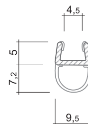
DD0149TR 2010 mm DD0150TR 2500 mm
