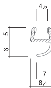
DD0157TR 2010 mm DD0158TR 2500 mm
