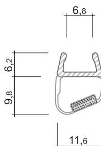
DD0120TR 2010 mm NS DD0121TR 2010 mm SN
