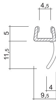
DD0147TR 2010 mm DD0148TR 2500 mm
