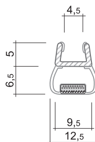
DD0147TR 2010 mm DD0148TR 2500 mm
