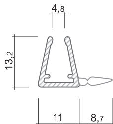
DD0090TR 2010 mm (see also DD0018TR)
