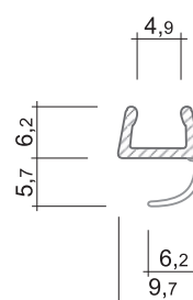
DD0100TR 2010 mm DD0167TR 2200 mm
