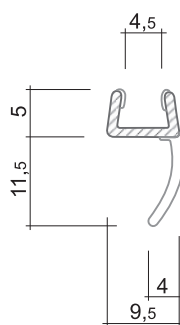
DD0147TR 2010 mm DD0148TR 2500 mm
