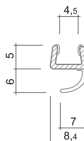
DD0153TR 2010 mm DD0154TR 2500 mm
