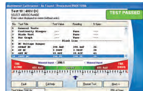
GRAPHICAL CALIBRATION
