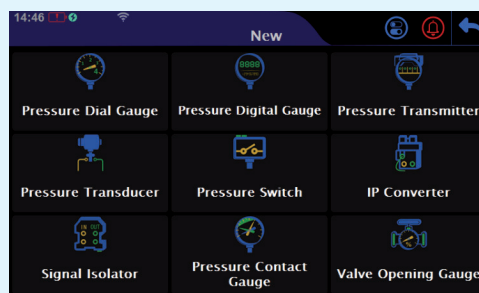
Task Menu
