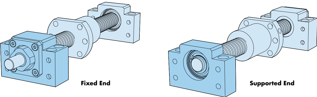
Illustration of Hepco ball screw fitted with Fixed End and Supported End bearing housings:
