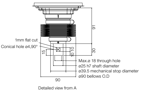
Flange (cleanroom)
