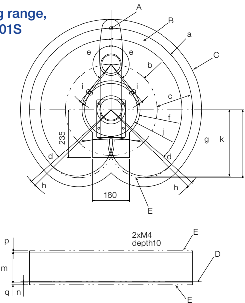
Working range, Epson SCARA LS3-B
