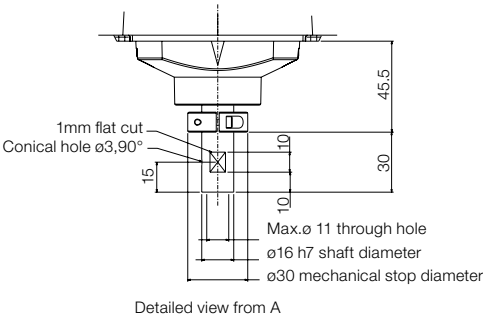
Flange (standard)
