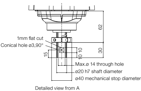
Flange (standard)
