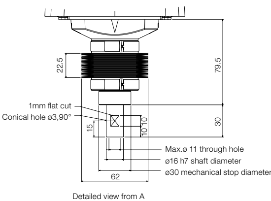
Flange (cleanroom)
