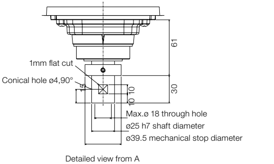
Flange (standard)
