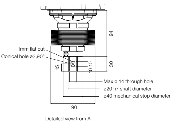
Flange (cleanroom)
