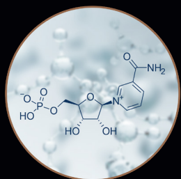
NMN (nicotinamide mononucleotide)
