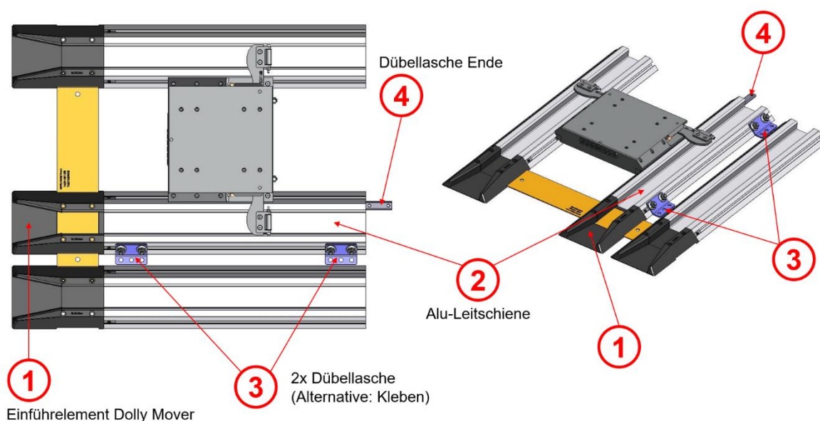
Fig. 1: Components for Dolly Mover®
