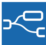
Node-RED™
