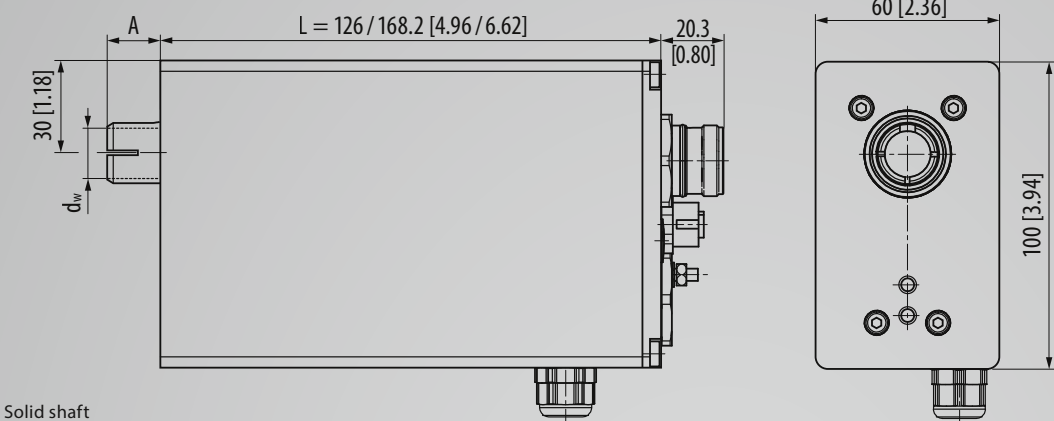
Solid shaft
