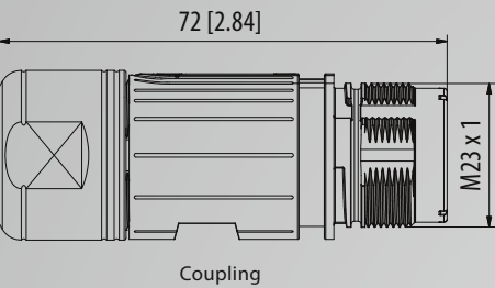
Connector type 23
