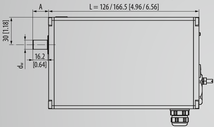
Solid shaft
