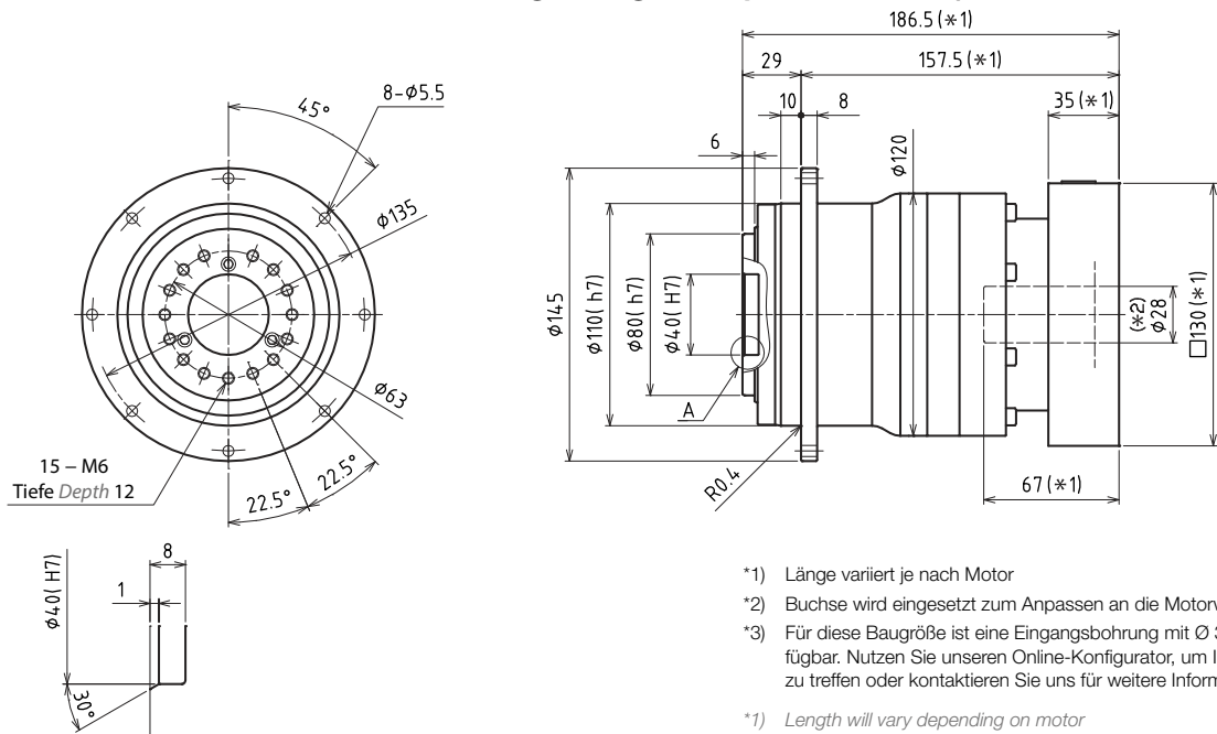
Detailansicht A Enlarged detail A
