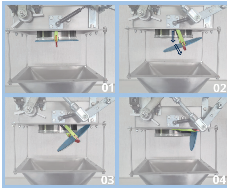
Fig. 2: Flap shutter mechanism
