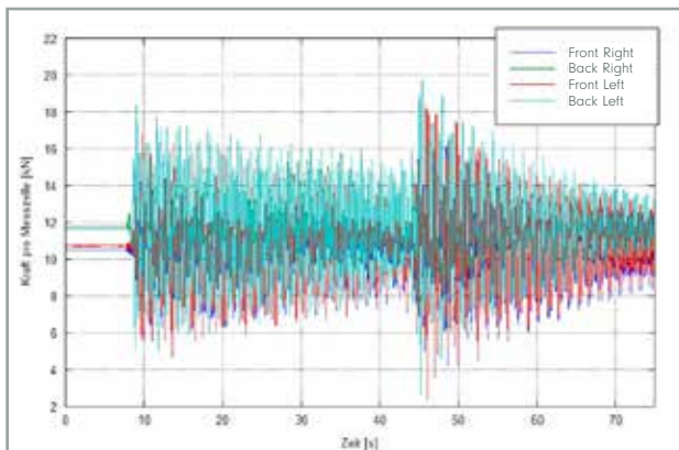
Abb 1 Conventional Steel Springs
