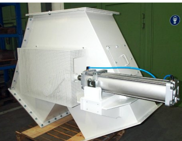
Distributor pneumatically driven
