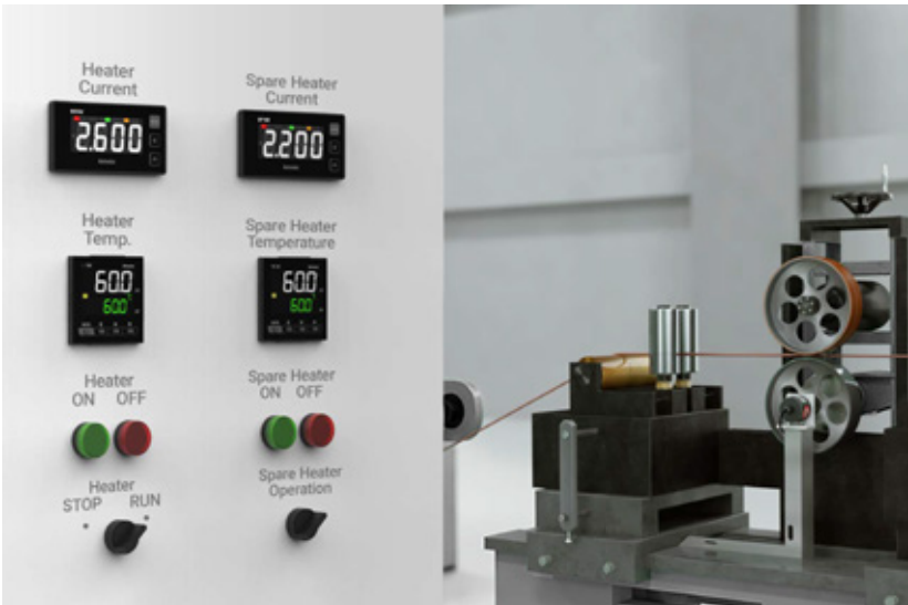
Wire Extrusion Molding Temperature controllers are used to control heat levels for raw material heating during wire extrusion molding process.
