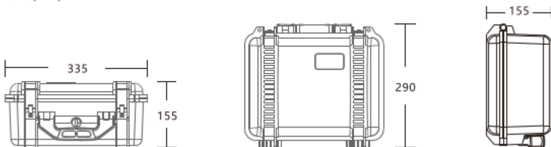
Dimensions(mm)
