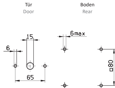
Bohrbilder Drillings
