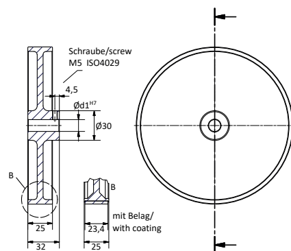
Measuring wheel FDA 500
