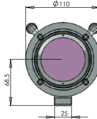
Dimensions industry protection housing „protection“ (IP65)
