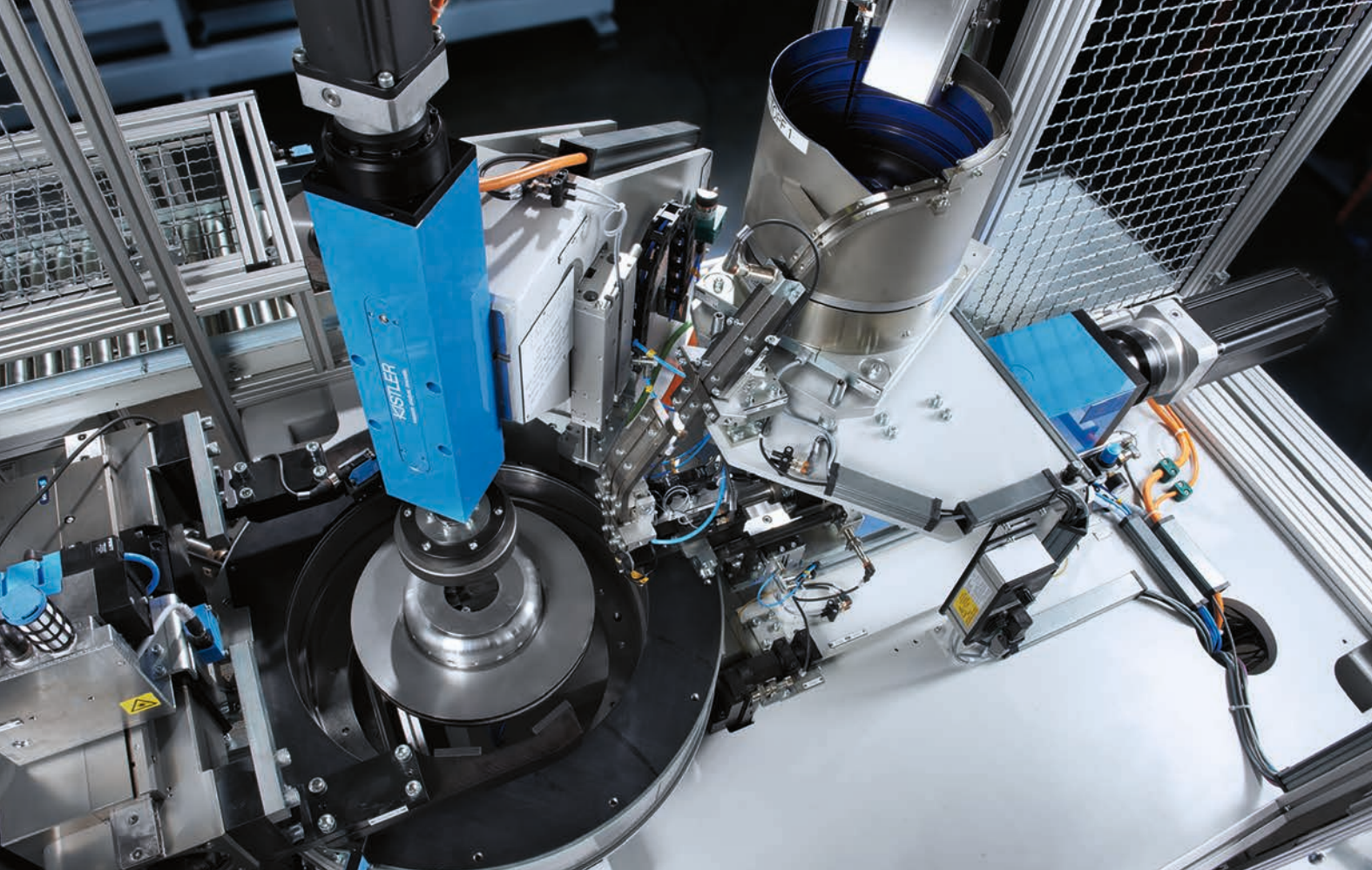
Application for riveting a lightweight brake disk with the help of force-displacement monitoring
