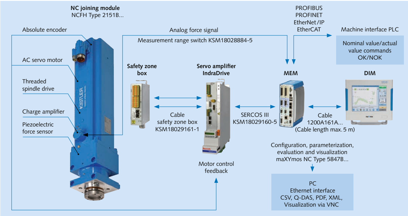
Operating principle of an NC joining system with NC joining module NCFH, Type 2151B... and maXYmos NC, Type 5847B...
