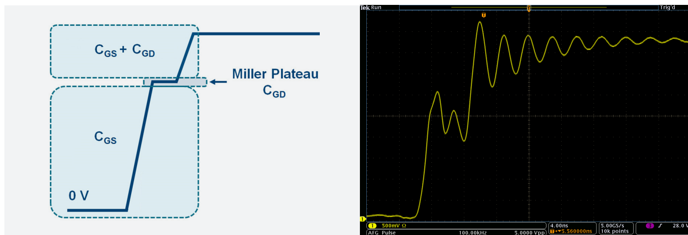
FIGURE 5. Comparison of the Tektronix IsoVu High-Side V_{GS} Output to Ideal.
