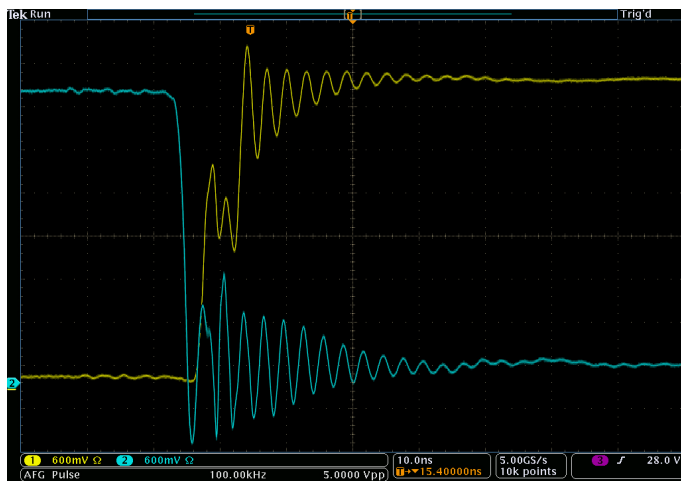
FIGURE 8. Interaction of the High-Side and Low-side Switches.
