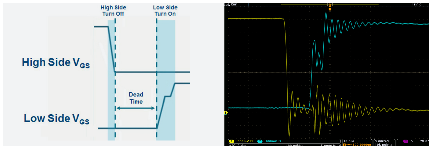
FIGURE 9. High-Side Turn Off, Low-Side Turn On, and Dead Time.
