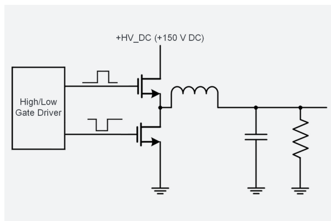
FIGURE 1. Half-Bridge Configuration.
