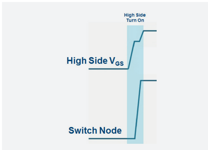
FIGURE 7. High-Side V_{GS} Turn On and Switch Node Compared to Ideal.
