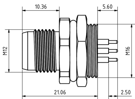
Stecker / Male
