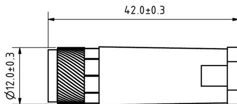
Type -21- Kupplung / Female
