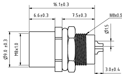
Kupplung / Female
