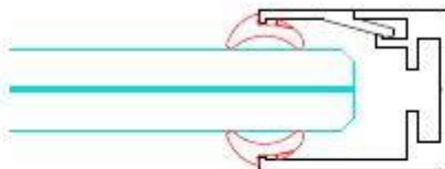
HORIZONTALE DOORSNEDE DETAIL (C) SCHAAL 1/1
