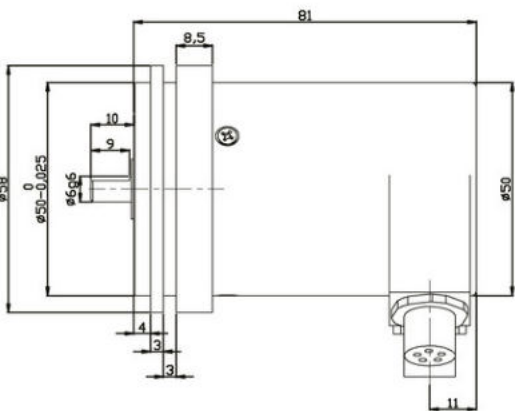
EAM58B Radial
