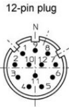
12-pin plug
