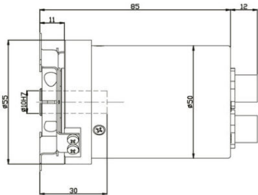
EAM58W Axial
