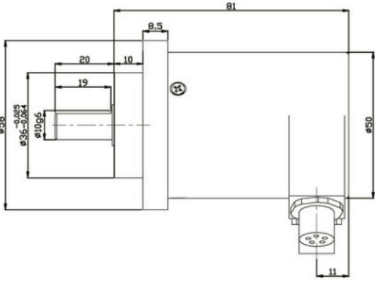
EAM58C Radial
