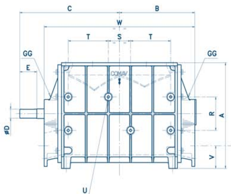
FRONTAL VIEW
