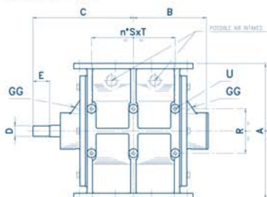
FRONTAL VIEW
