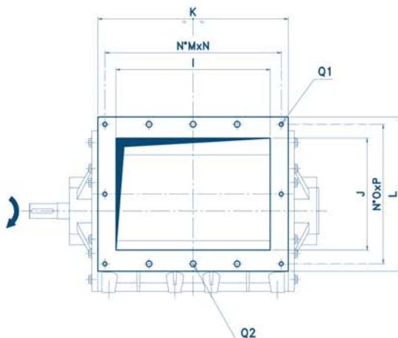
FLANGING VIEW
