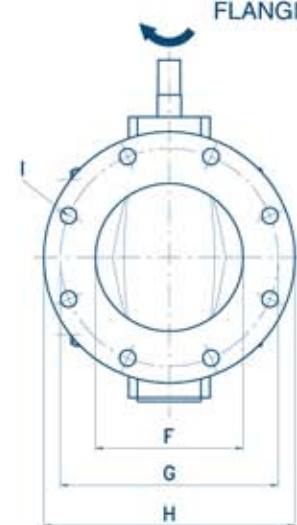
FLANGING VIEW
