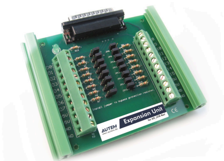
Expansion Unit for AD_USB-Box (scope of supply)
