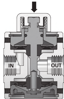
250 NO, Actuated
