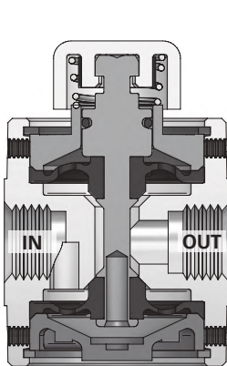
250 NC, Unactuated
