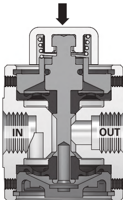
250 NC, Actuated
