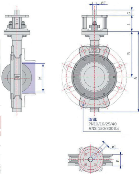
Wafer
