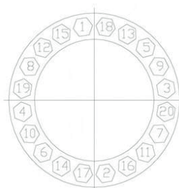
FASTENING SCREWS SEQUENCE(Picture 9)
