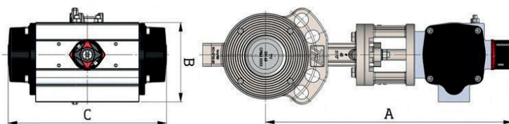
Colossus with Simple Effect Actuator (ASR)
