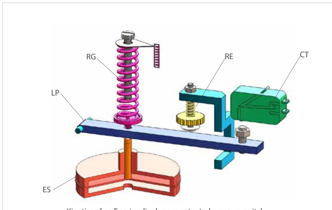
Kinetics of an F series diaphragm-actuated pressure switch
