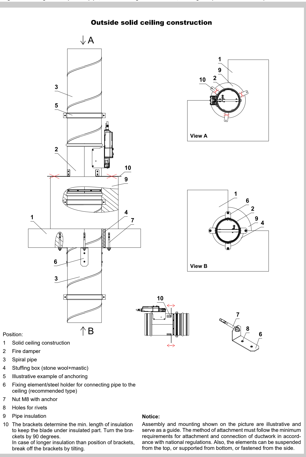
Fig. 40 Fixing fire damper and pipe, outside ceiling with insulation, stuffing box (stone wool + mastic)
