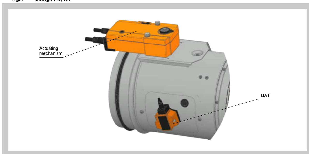
Fig. 7 Design .40, .50
