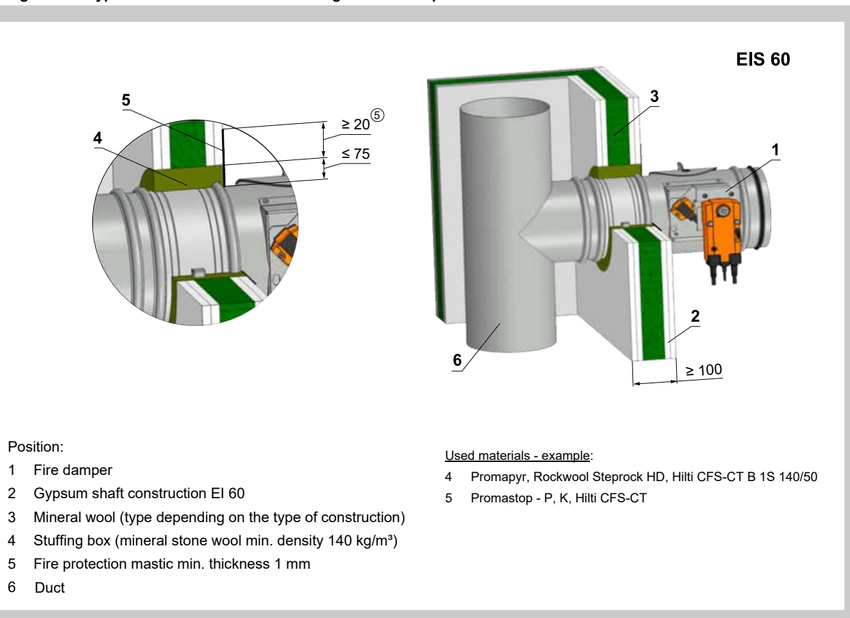
Fig. 35 Gypsum shaft construction - stuffing box and fire protection mastic
