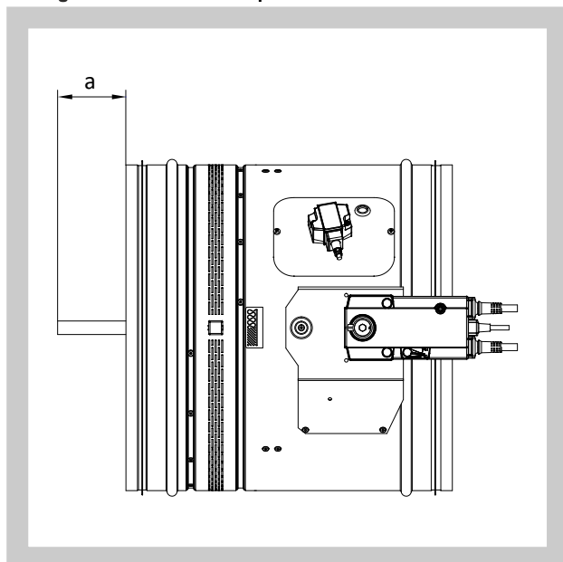
Fig. 17 Blade overlaps
