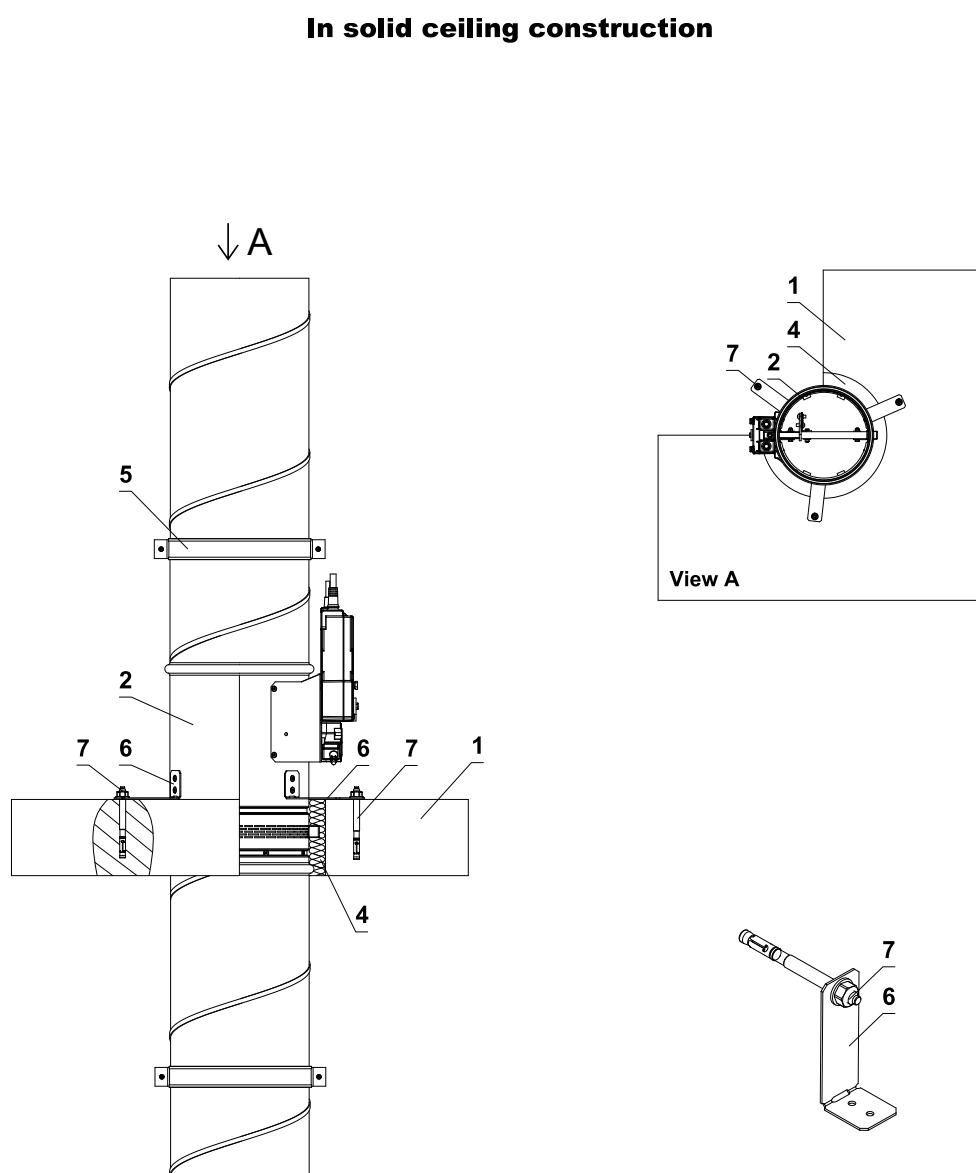
Fig. 38 Fixing fire damper to the ceiling with stuffing box (stone wool + mastic)
