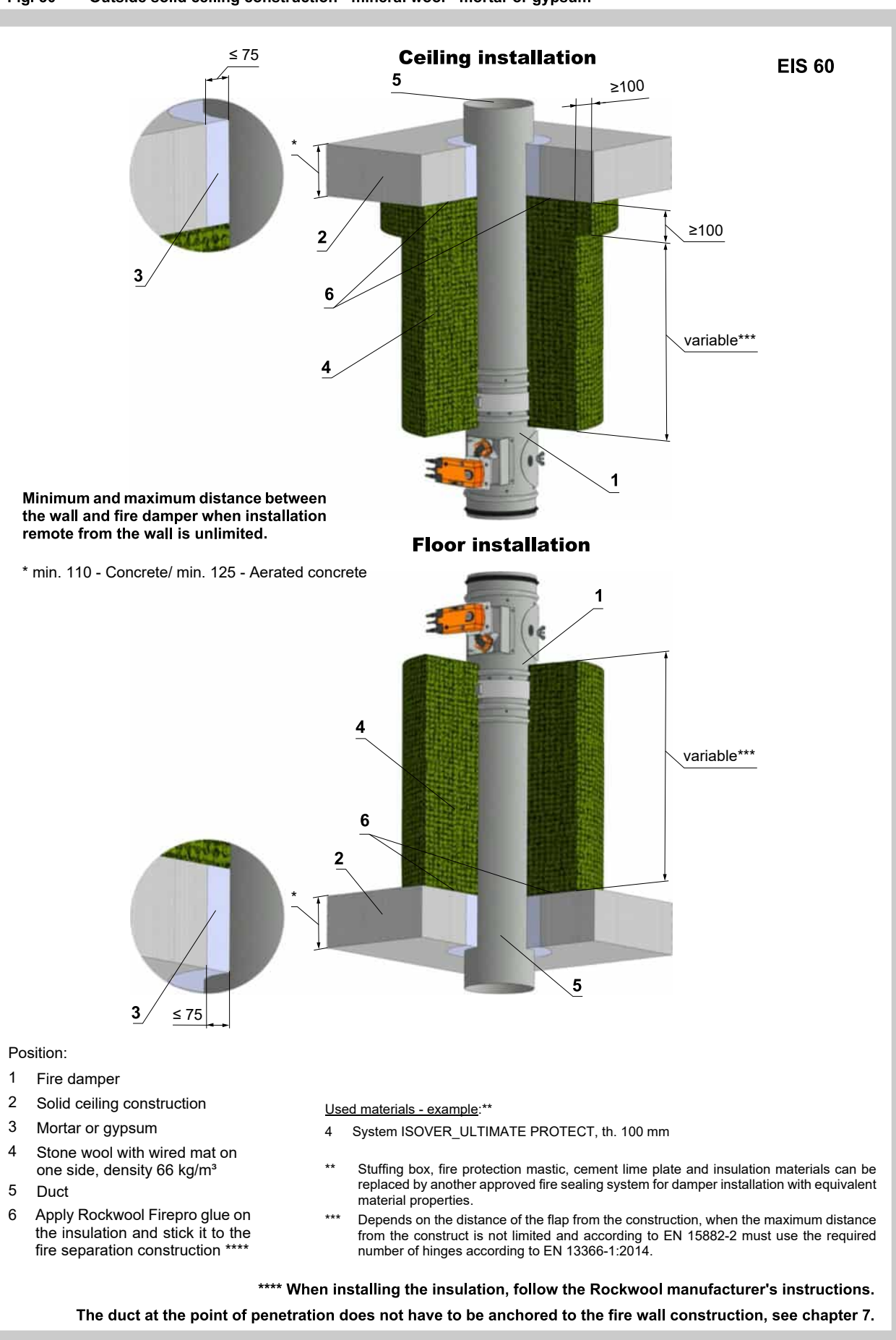
Fig. 30 Outside solid ceiling construction - mineral wool - mortar or gypsum
