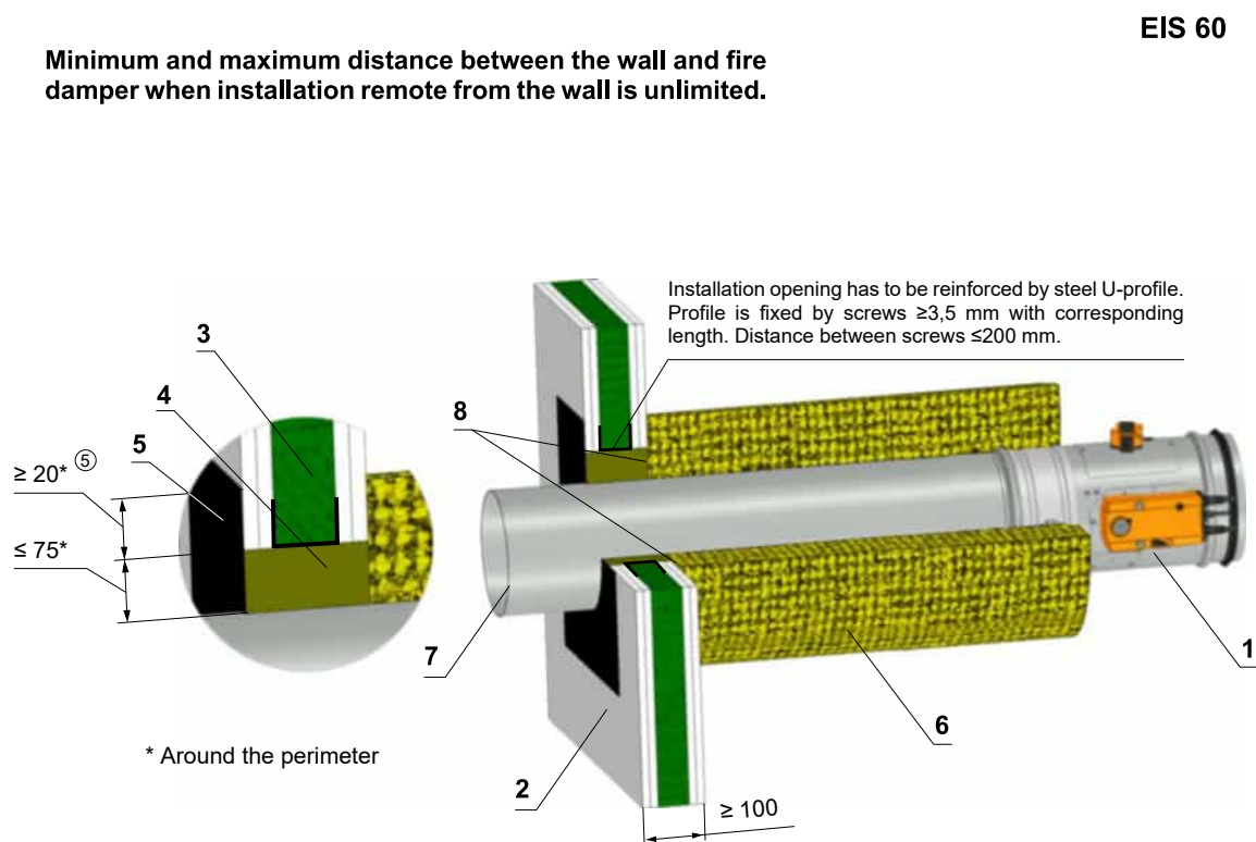
Fig. 27 Outside gypsum wall construction - mineral wool - stuffing box and fire protection mastic
