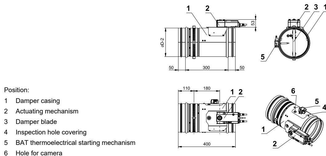
Fig. 16 Fire damper with installation holders
