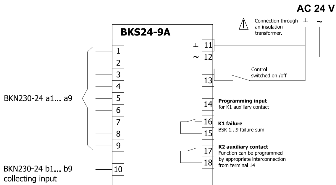
Fig. 13 Communication and control device BKS 24-9A
