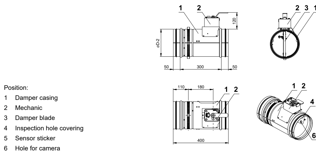
Fig. 15 Design with actuating mechanism
