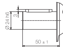
Passfeder (optional)
