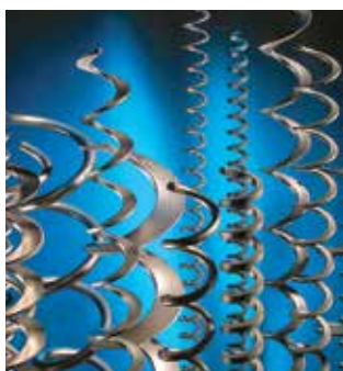
Flexicon stocks an unequalled selection of standard and custom flexible screws to match the flow characteristics of each bulk material, yielding the greatest conveying efficiency.
