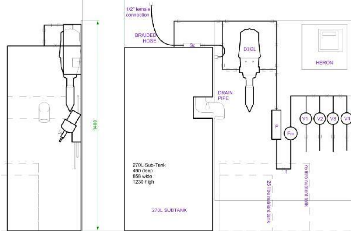
Typical Irrigation Rig for living wall over 100m2
