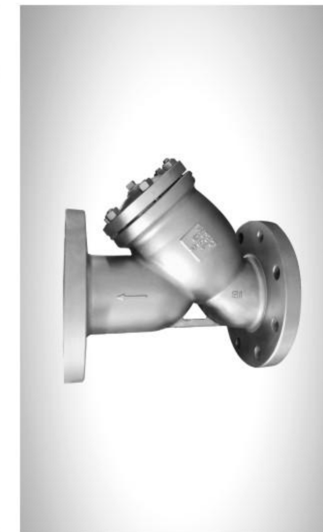
Flanged Y Type Strainer Size:1/2"-12" Material:SS304/SS316/WCB Pressure:150LB/300LB
