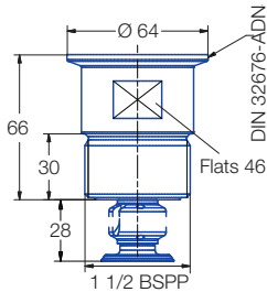
Male thread
