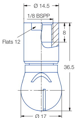
Female thread
