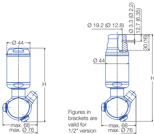
Female thread
