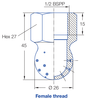
Female thread
