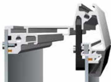
Front panel installation from rear
