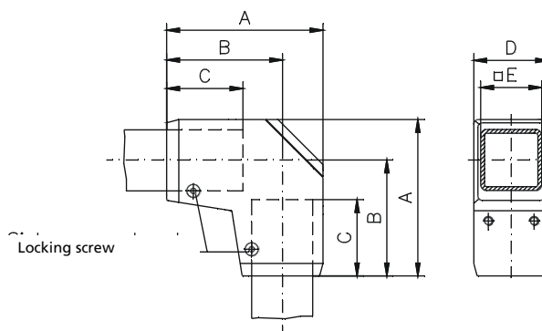
Type Order No. Weight (g) A B C D E 50/2 49.51 80 00 4720 154 115 80 74 50 60/2 49.61 80 00 6200 172 128 90 84 60 80/2 49.81 80 00 9000 210 157 105 98 80
