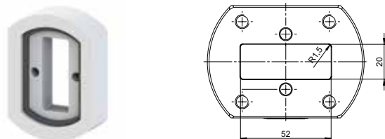
Adapter GTS
