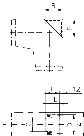
Type Order No. Weight (g) A B C D E F 50/2 49.51 80 10 300 74 60 36 54 29 38 60/2 49.61 80 10 360 84 65 40 62 32 43 80/2 49.81 80 10 400 98 76 54 82 42 54
