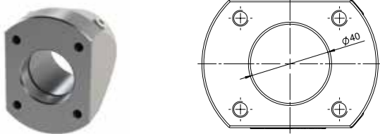
Adapter GT 48/2
