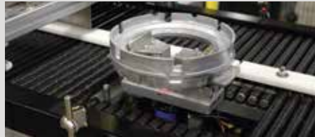
6. ORIENTING Ensures gentle product handling for organized conveying including product turning, rotating, inverting or positioning.
