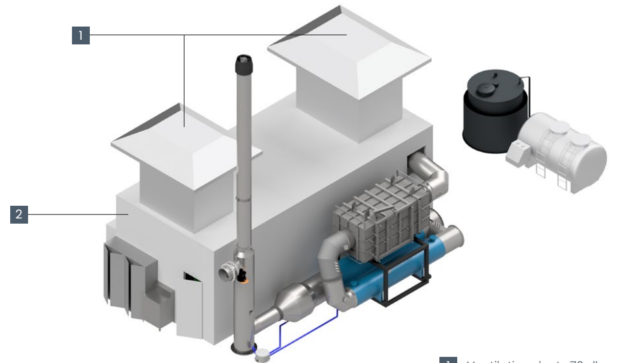
Exterior view of the modular system (standard layout)
