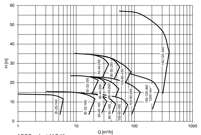
1800 min⁻¹/60 Hz
