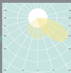
PG 60 asymmetrical reflector system
