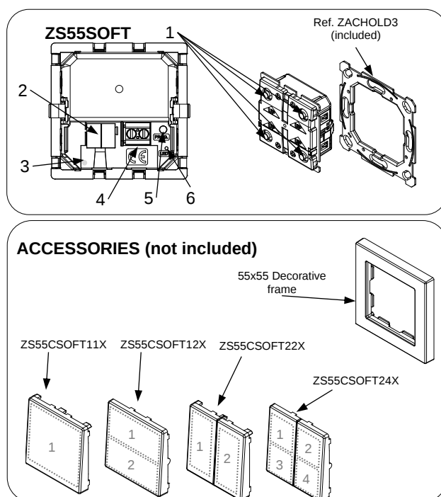
Figure 1: Soft Push button 55x55
