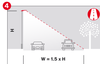
ST1.5a – For very wide roads; lighting class M; e.g. roads with adjacent areas, parking lots
